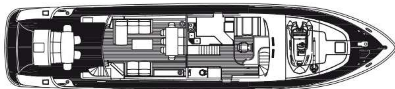
Main deck
